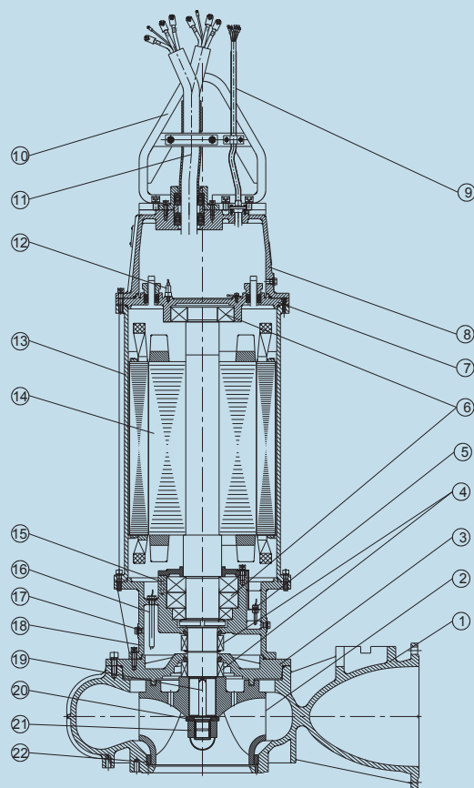
Structure Diagram
