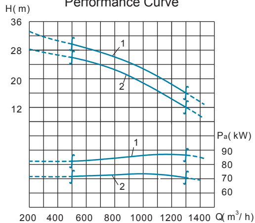
Performance Curve
