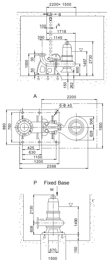
Installation Diagram
