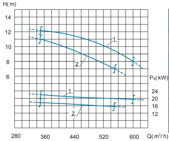
Performance Curve
