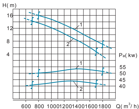
Performance Curve
