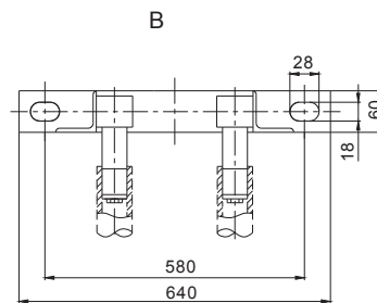
Z Automatic Coupling Installation
