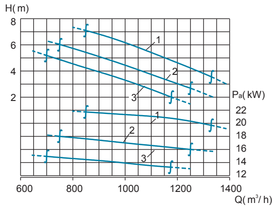
Performance Curve
