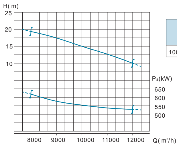
Performance Curve
