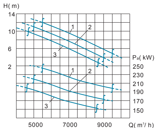
Performance Curve
