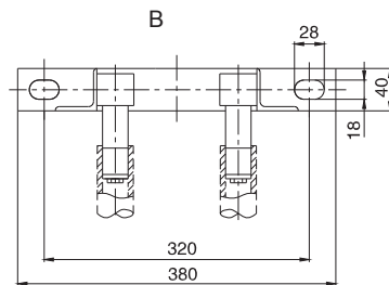
Z Automatic Coupling Installation
