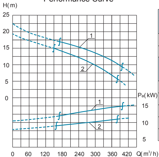
Performance Curve
