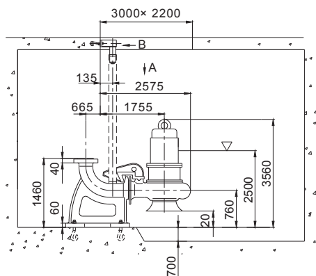
Installation Diagram
