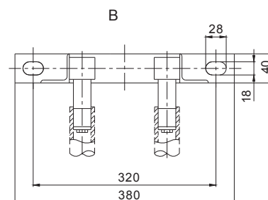
Z Automatic Coupling Installation
