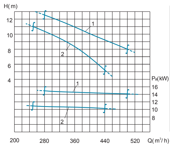
Performance Curve
