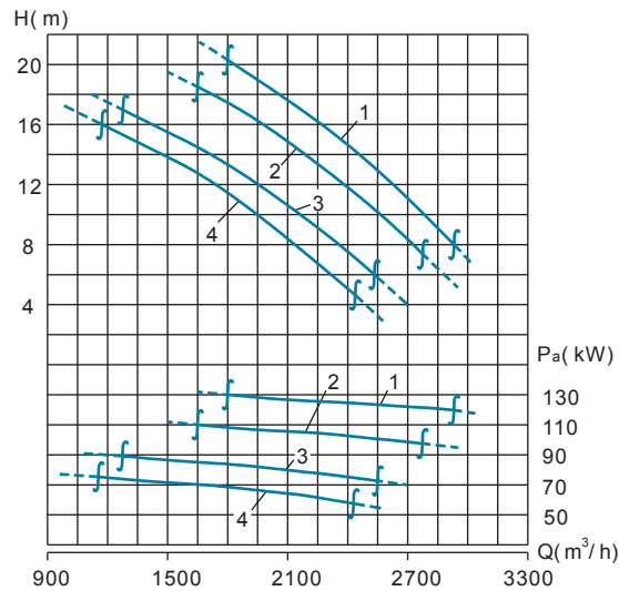
Performance Curve
