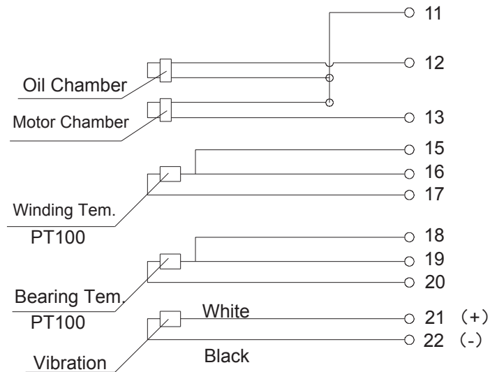
Y290-Y445 Schematic diagram of YVC12 x 1 wiring of the control cable
