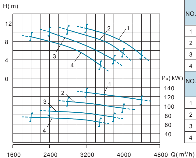
Performance Curve
