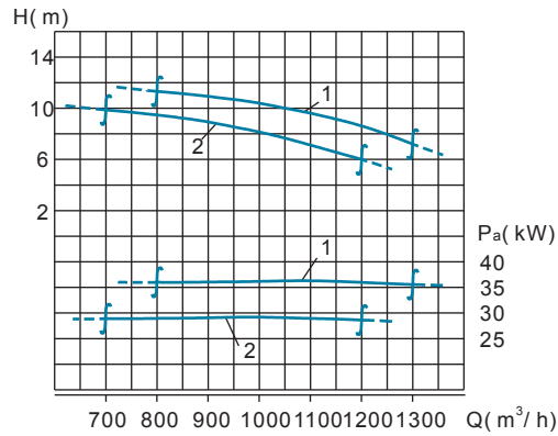
Performance Curve
