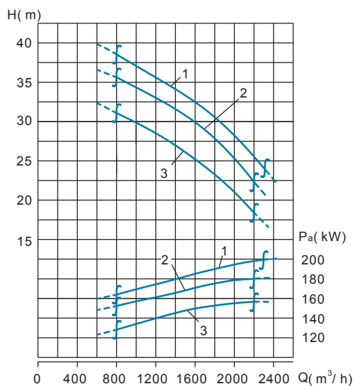
Performance Curve
