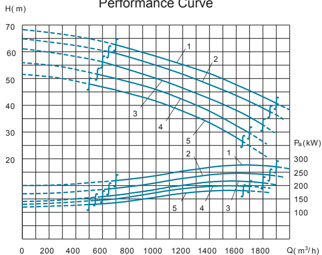
Performance Curve
