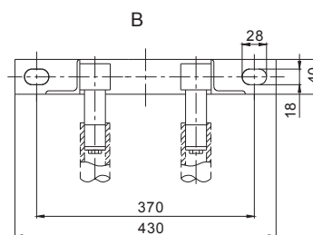
Z Automatic Coupling Installation
