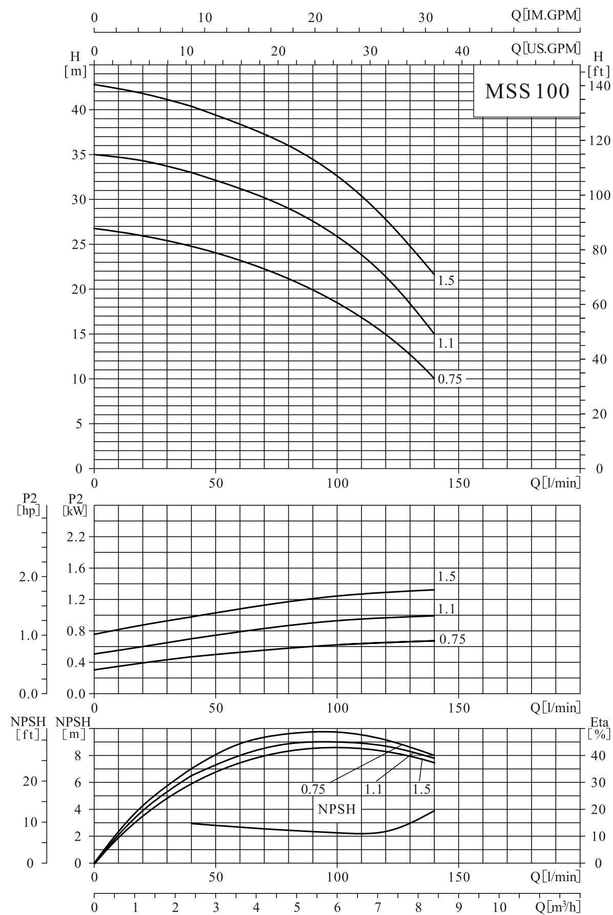
MSS100 Performance curve
