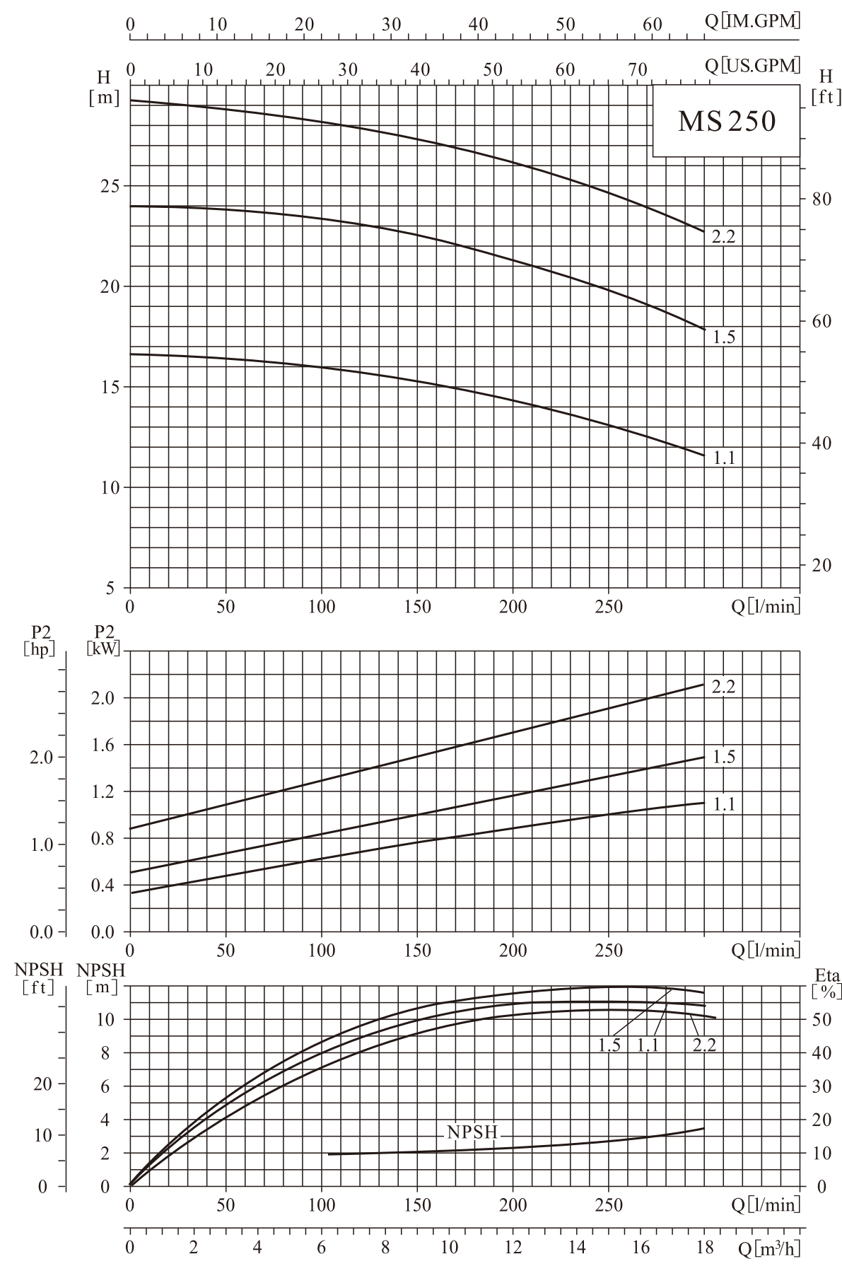
MS250 Performance curve
