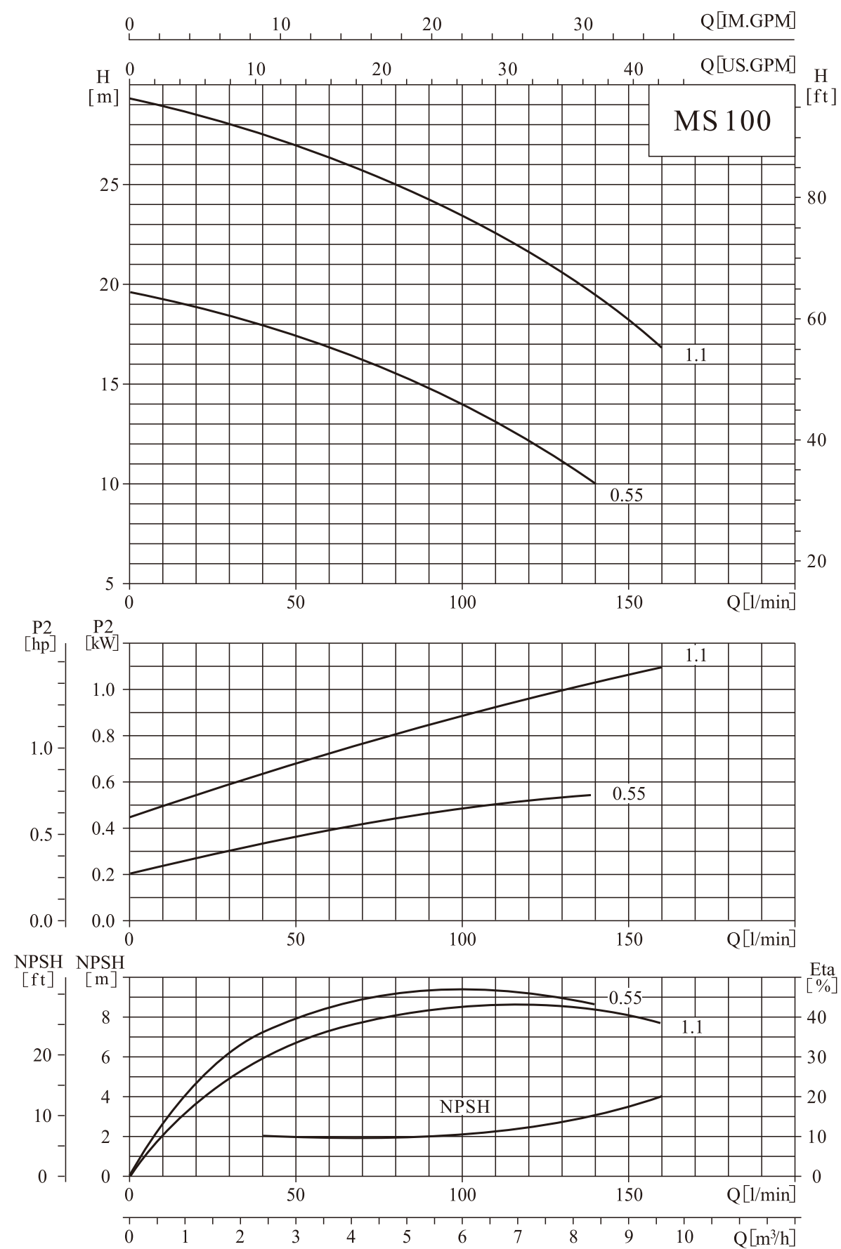
MS100 Performance curve
