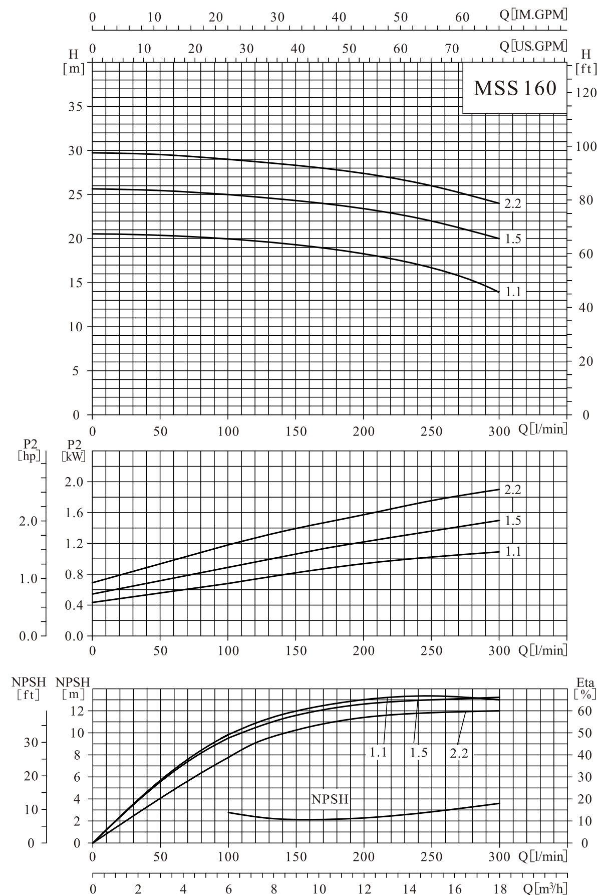
MSS160 Performance curve
