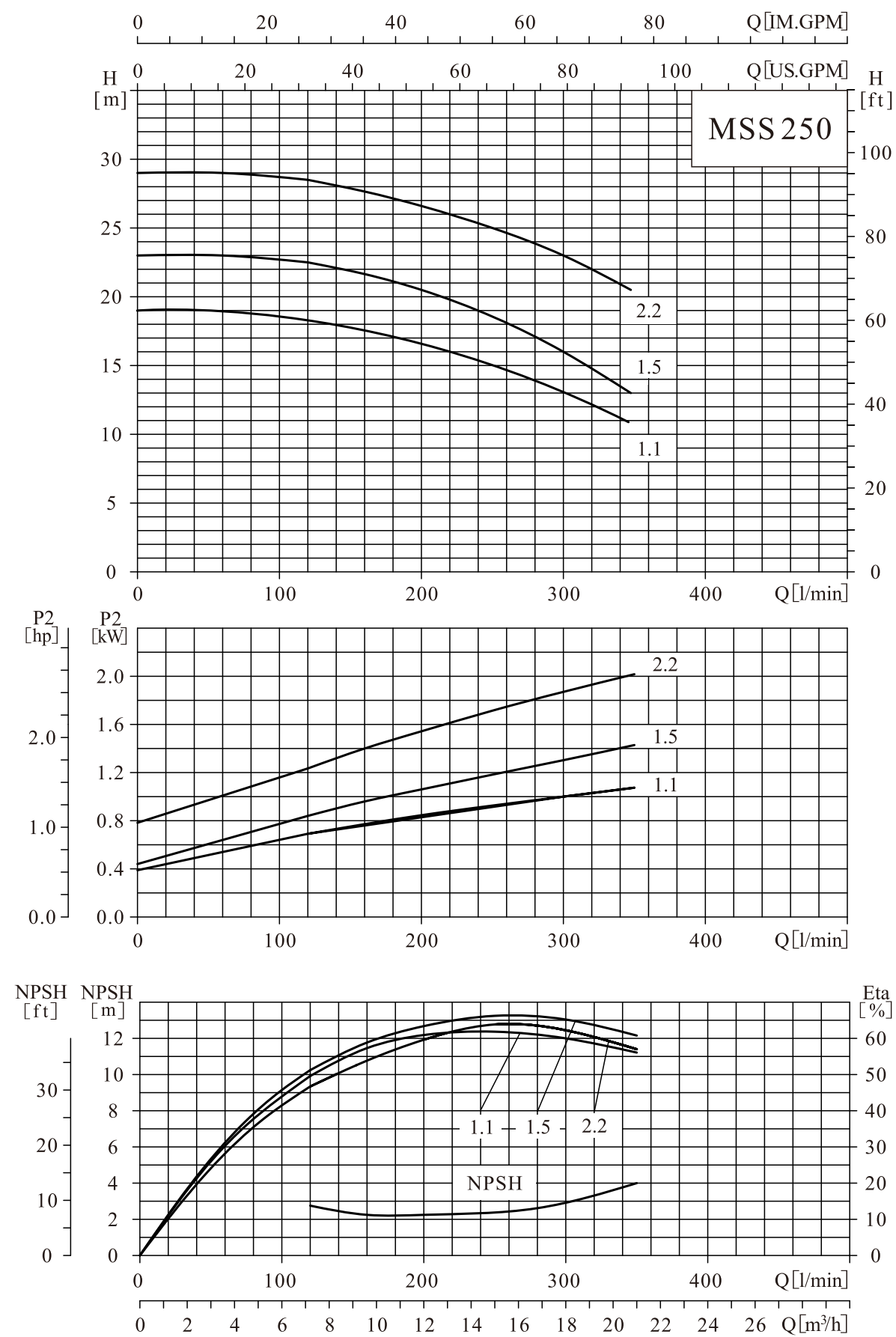
MSS250 Performance curve
