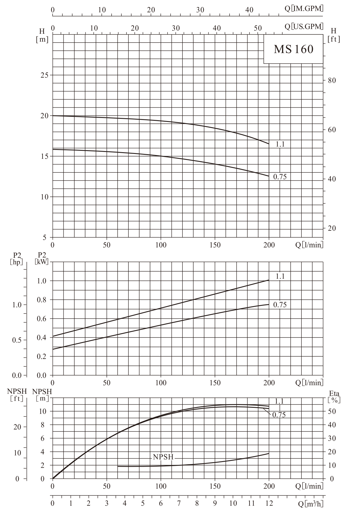
MS160 Performance curve
