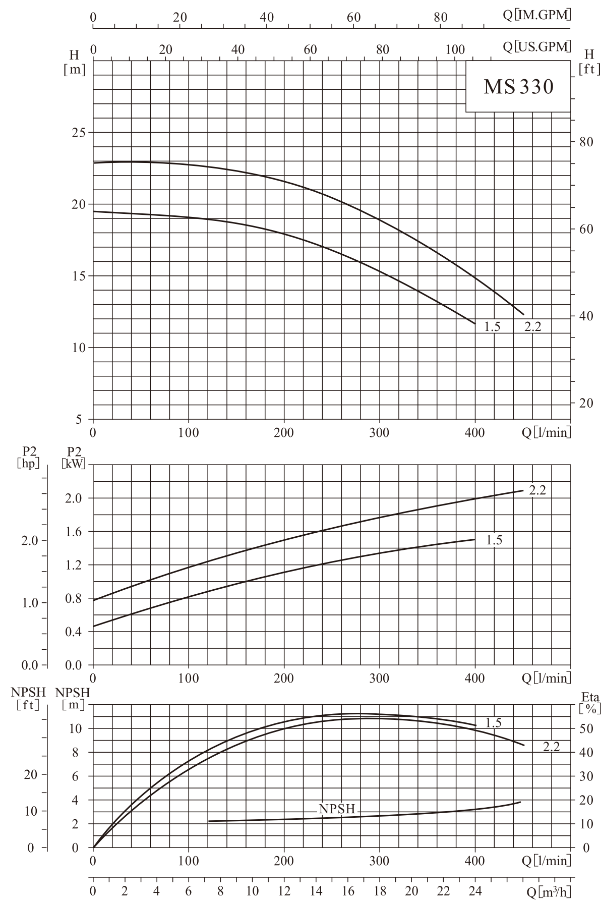
MS330 Performance curve
