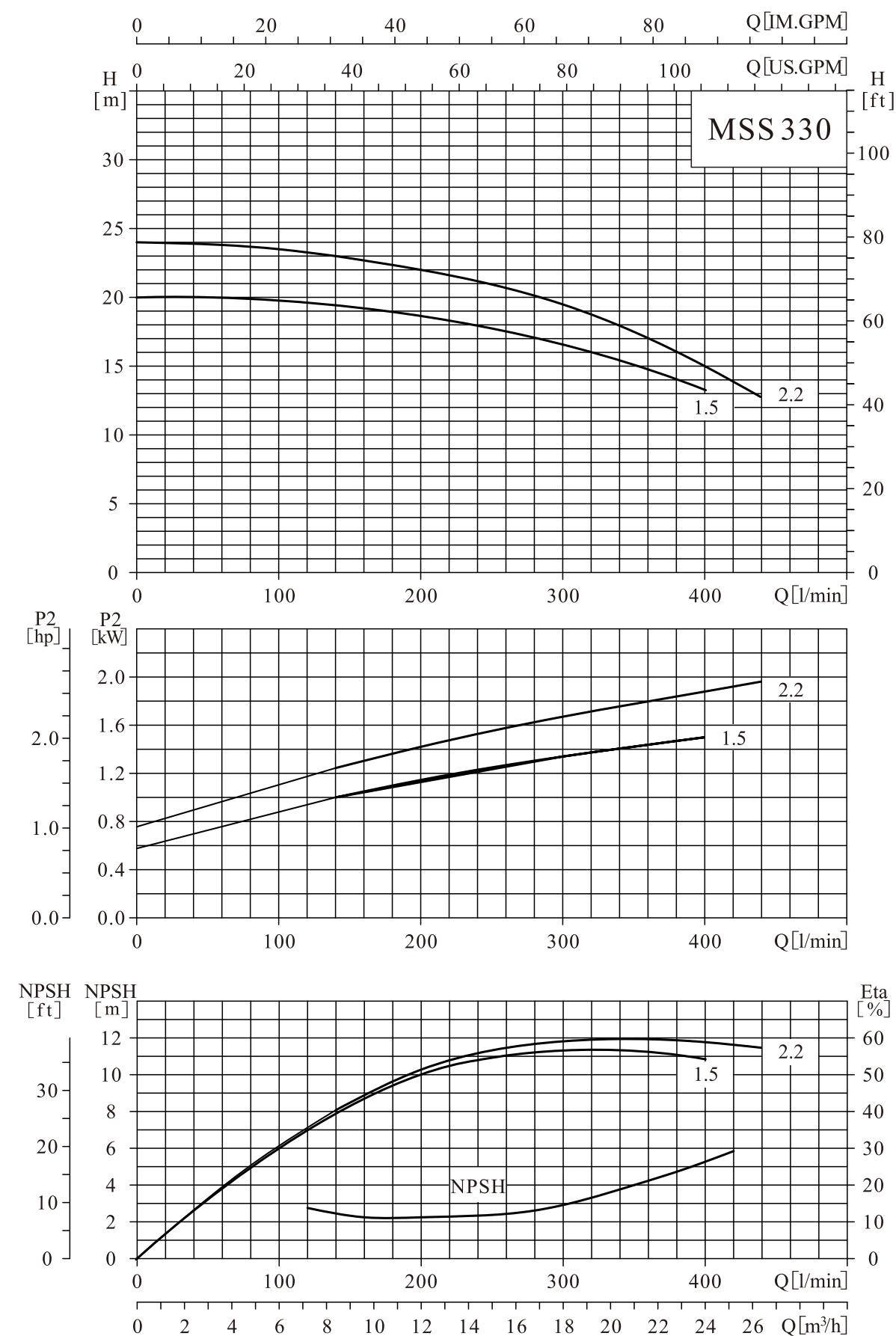
MSS330 Performance curve
