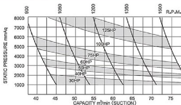
MODEL: DN-300A(LT-300A)
