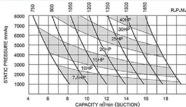
MODEL: DN-125(LT-125)
