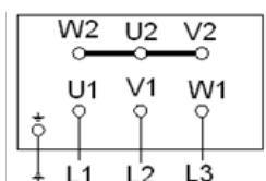
Diagram 3: Connection
