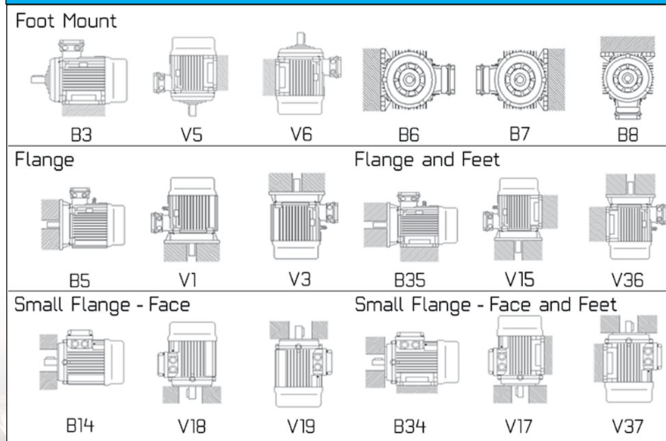
Diagram 2: Mounting Arrangements
